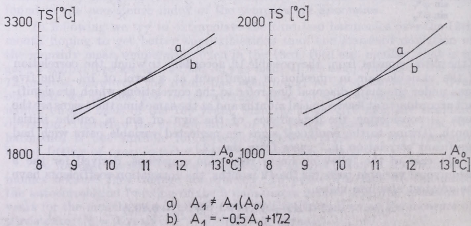
Figure 1. Dependence of the temperature sum on the yearly mean without feedback (a) and with feedback (b) for T_0 = 5^\circ\text{C} (on the left) and T_0 = 10^\circ\text{C} (on the right) respectively
