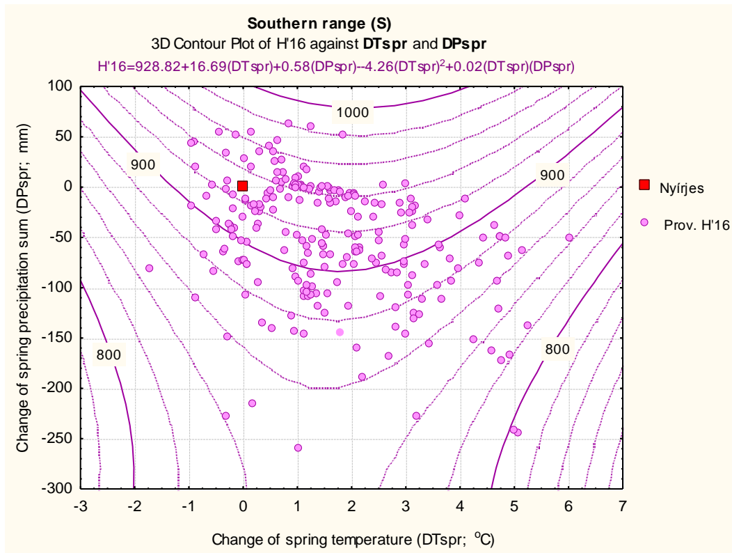
Figure 34b. Contour plot of multiple regression of adjusted height of Southern provenances at age16 ( H'16 ; cm) in Nyirjes versus ecological distances of transfer [spring precipitation change ( DP_{spr} ) and spring temperature change ( DT_{spr} )]. The reference position of Nyirjes is marked with a red quadrate. For statistical data see table in Figure 34a
