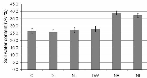
Figure 5. Soil water content % (v/v) in 0-15 cm depth. (average of the data between 2002-2005)
