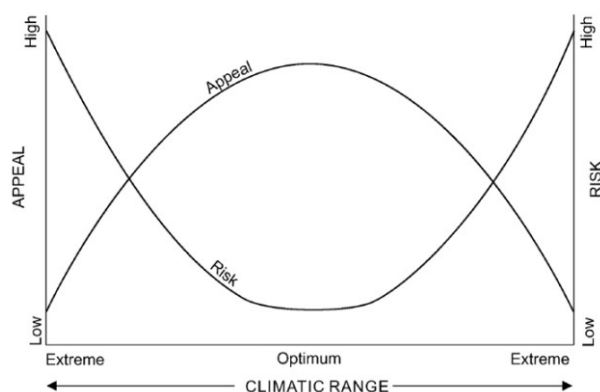
Fig. 1 Schematic representation of relationship between a climatic range and tourism potential. The climate potential of a particular location is a function of its climate and of the risks that weather may impose. (de Freitas, 2003 after Perry, 1997).
