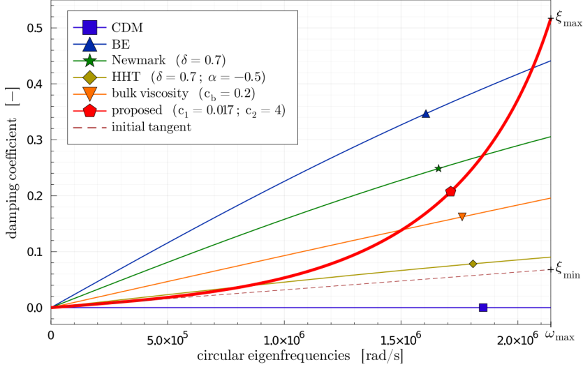
Damping ratio for the examined methods
