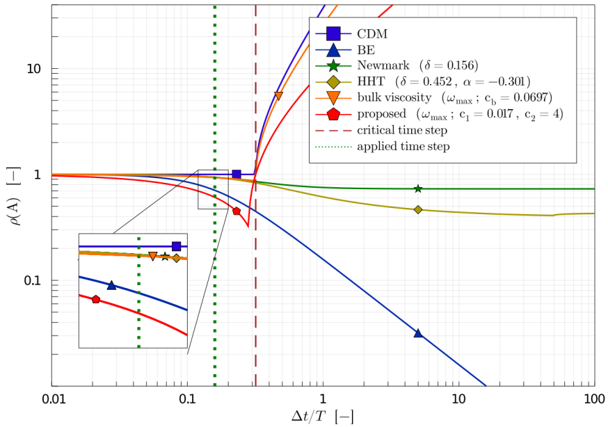
Figure 5 Spectral radii of the examined methods
