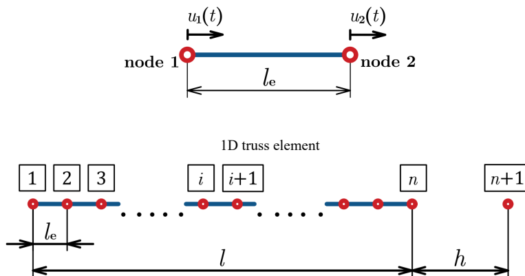
FE model
