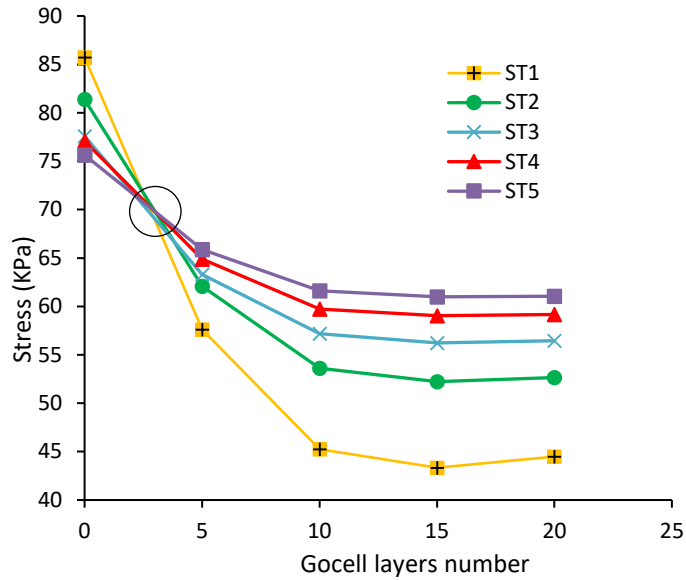
Figure 5 Stress-geocell layers number curves for different soil types
