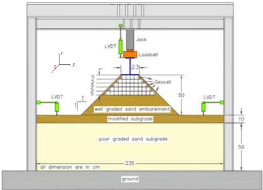
Figure 1 The laboratory geocell-reinforced embankment including 5 geocell layers [25]
