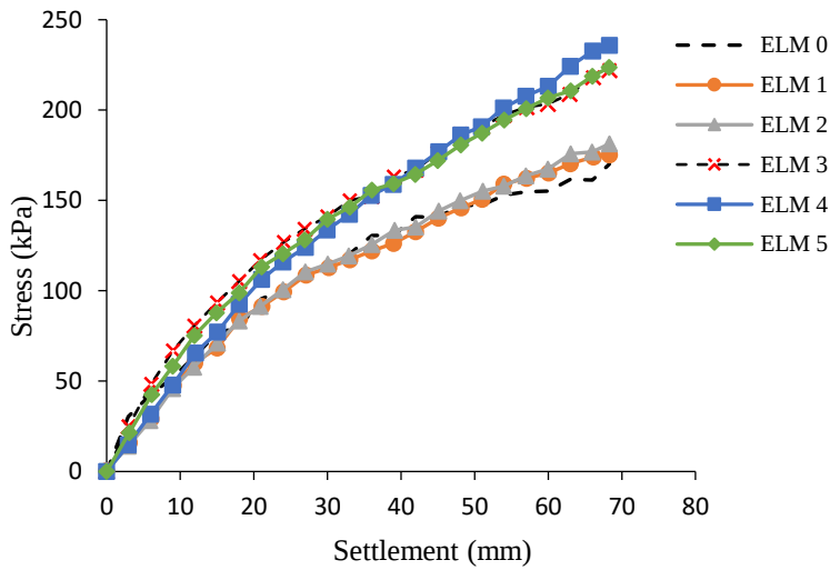
Figure 6 Load-settlement behavior of experimental geocell-reinforced and reference models [19]
