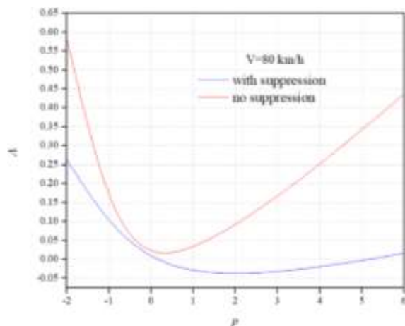
Figure 8 Stability boundaries in the lateral direction
