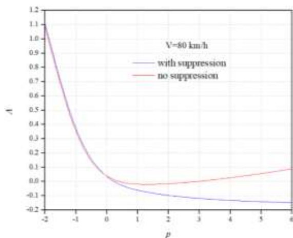
Figure 9 Stability boundaries in the longitudinal direction
