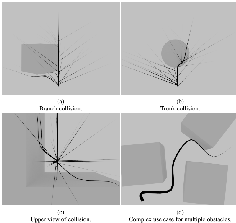
Figure 5 Validation of the collision detector.
