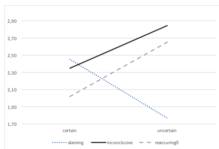
Figure 8 Text evaluations
