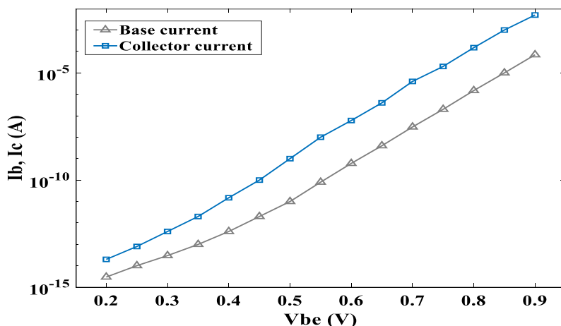
Figure 3 Gummel plot (source: [28])
