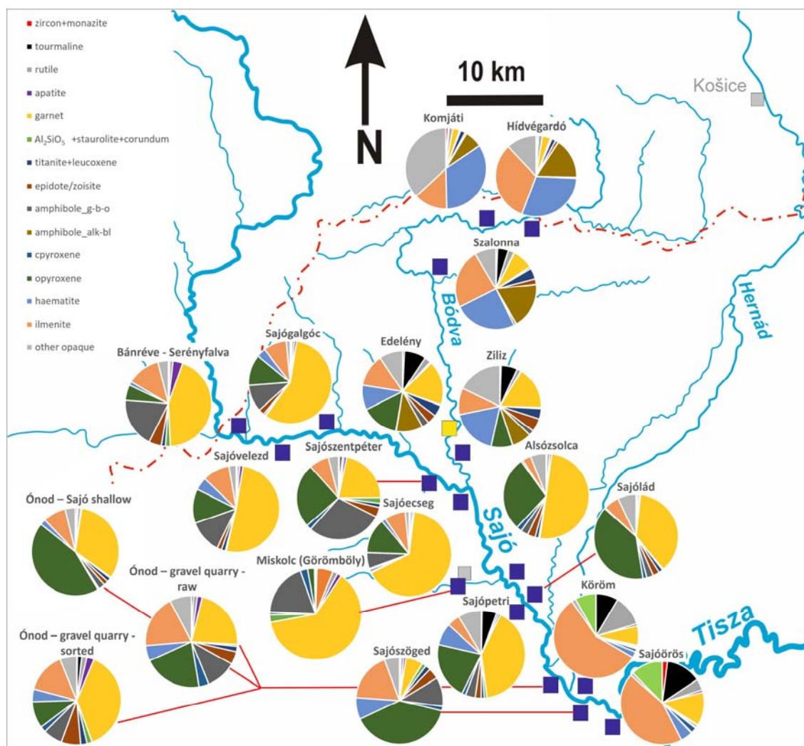
Fig. 3.: Heavy mineral distribution of sediments from the Bódva and Sajó valleys (the interest of our study, the archaeological site is indicated with yellow square). Note that values of the pie diagrams are not equivalent with the values in Table 1, but normalized to 100% without 'biotite', 'chlorite', the 'light minerals', 'lithofragments' and 'undetermined altered grains'. Abbreviations in the figure are pyroxene: clinopyroxene, opyroxene: orthopyroxene, amphibole_g-b-o: green-brown-oxyamphibole, amphibole_alk-bl: alkaline-blue amphibole.
