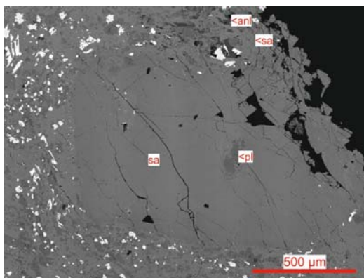
Fig 10.: BSE image of NUH-H1 phonolite on almost the same territory as in Fig. 8 . Mineral abbreviations: sa – sanidine, pl – plagioclase, anl – analcime
