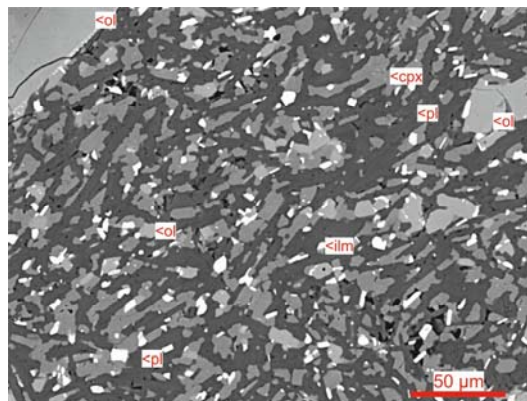
Fig. 7.: Groundmass of NUH-V1 basalt in BSE image. Abbreviations: cpx – clinopyroxene, ilm – ilmenite, ol – olivine, pl – plagioclase
