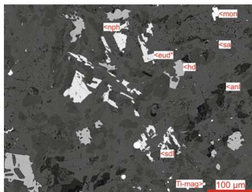
Fig. 11.: Groundmass of NUH-H1 phonolite flake in BSE image. Abbreviations: anl – analcime, eud* - eudialyte group mineral, hd – hedenbergite, mon – monazite, nph – nepheline, sa – sanidine, sdl – sodalite, Ti-mag – titanomagnetite
