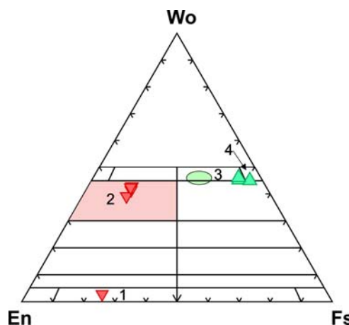
Fig 13.: Pyroxene composition of NUH-V1 basalt (red triangles) and NUH-H1 phonolite (green triangles) flakes. Basaltic sample contains clinopyroxene (2: Mg-rich augite) and – as inclusions in olivine - orthopyroxene (1: Ferroan-enstatite), whereas phonolite contains only clinopyroxene (3: Mg-hedenbergite, 4: hedenbergite). For comparison compositional range of clinopyroxenes of peralkaline phonolites from Ua Pou (pale green ellipsoide) and Tekao tholeiites of Nuku Hiva (pale red rectangle) are shown (based on Legendre et al. 2005a and 2005b, respectively).
